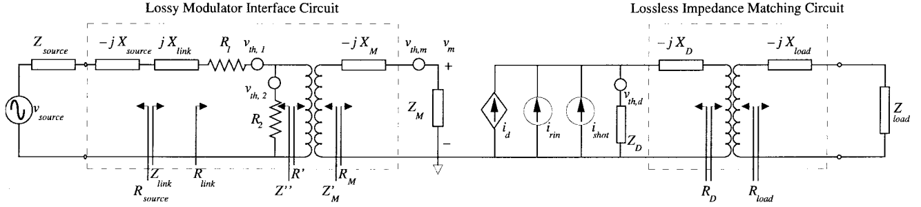
Fig. 3. Equivalent circuit for an intensity-modulation/direct-detection optical link with arbitrary input impedance Z_{\text{link}} , and resistors R_1 and R_2 to simulate loss in the modulator interface circuit.
