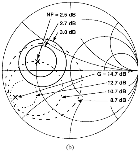
Fig. 5. (a) Analytically determined constant- G and constant-NF circles on a Smith chart plot of the transformed source impedance Z'_M presented to the modulator in the experimental amplifierless link. (b) Analogous constant- G and constant-NF circles for an example bipolar transistor. 1
