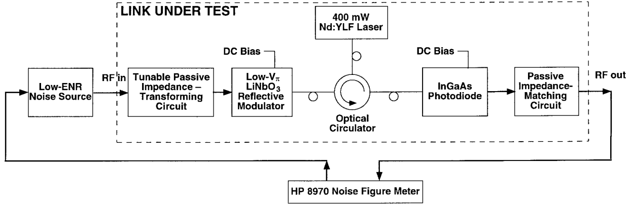
Fig. 4. Setup for measuring the NF of the experimental amplifierless link with tunable input impedance.
