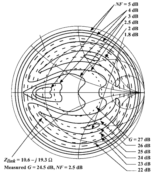
Fig. 6. Conformal mapping of the constant- G and constant-NF circles of Fig. 5(a) from Z'_M -space into Z_{\text{link}} space. The impedance where we measured G = 24.5 dB and NF = 2.5 dB is also shown.
