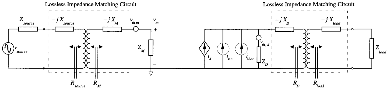
Fig. 1. Equivalent circuit of an intensity modulation/direct-detection optical link with perfect lossless input and output impedance-matching circuits.
